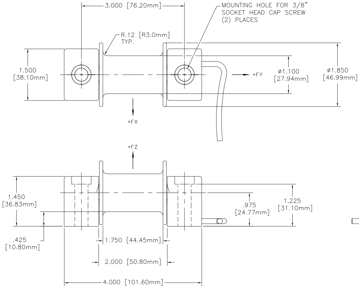
MODEL 5315 BELT ANCHOR LOAD CELL
